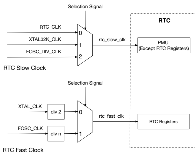
Figure 9-3. RTC Clocks
