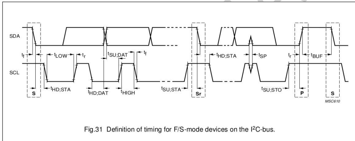
Figure 26-3. I2C Protocol Timing (Cited from Fig.31 in The I2C-bus specification Version 2.1 )
