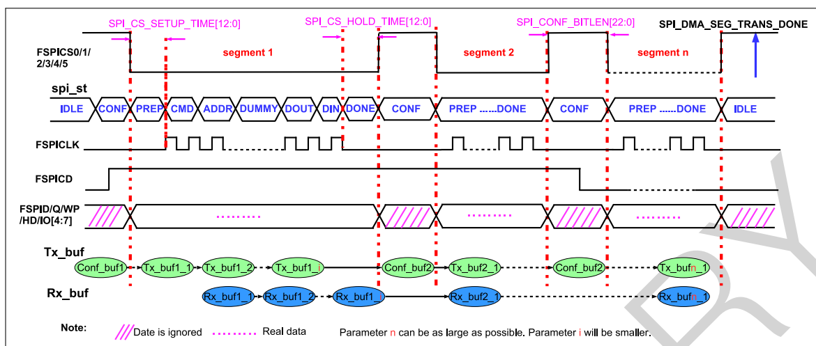
Figure 25-10. Configurable Segmented Transfer in DMA-Controlled Master Mode
