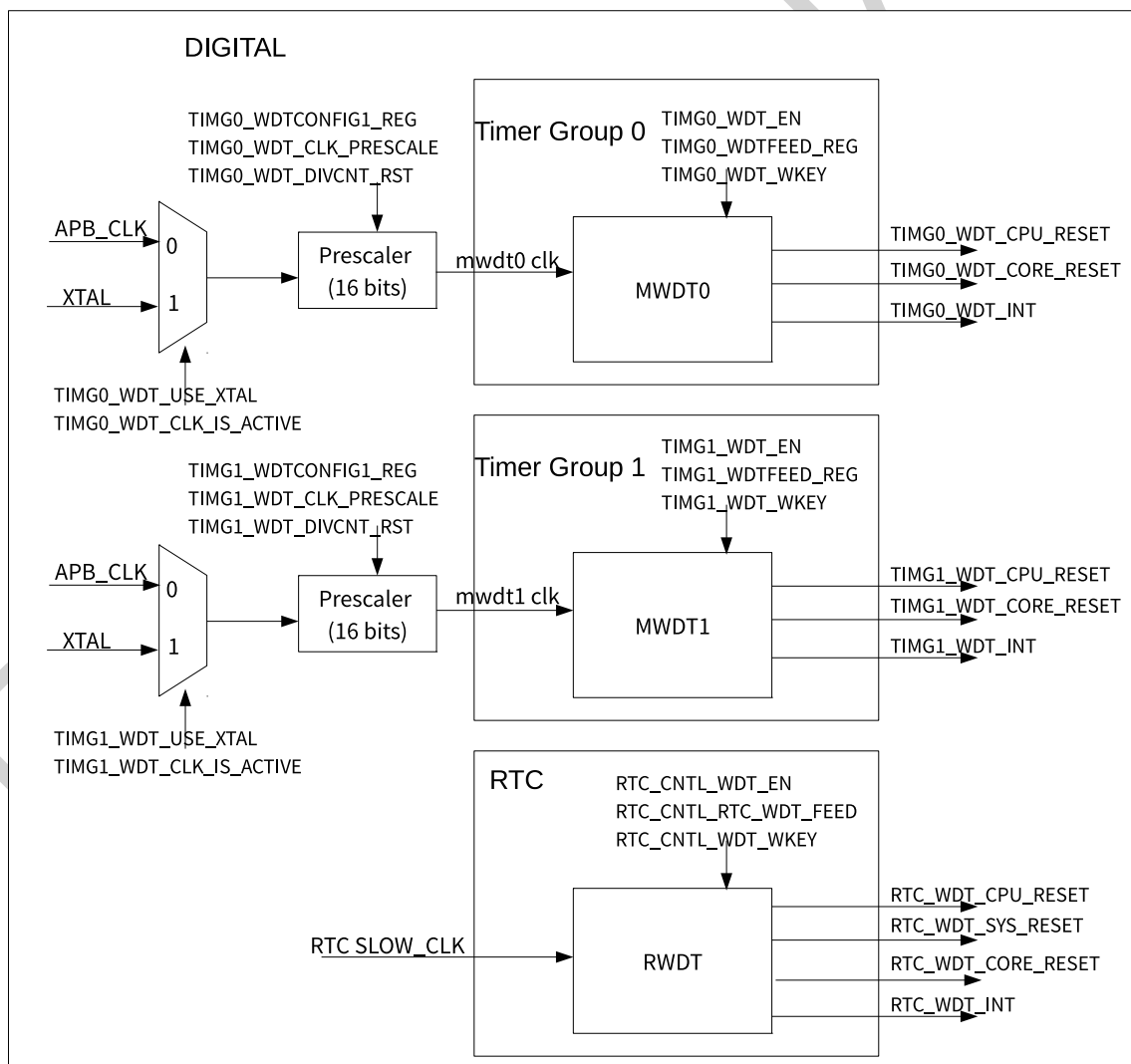
Figure 12-2. Watchdog Timers in ESP32-C3
