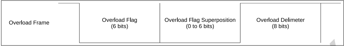
Figure 29-3. Fields of an Overload Frame
