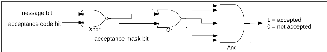
Figure 29-7. Acceptance Filter
