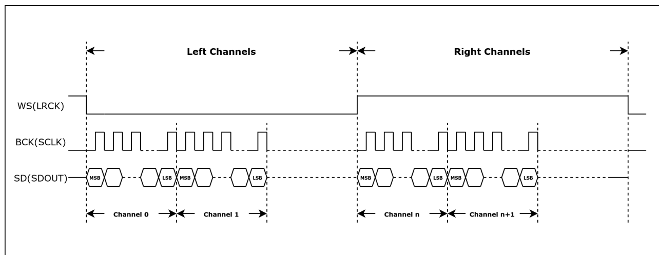
Figure 27-3. TDM MSB Alignment Standard Timing Diagram
