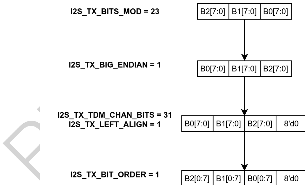
Figure 27-7. TX Data Format Control
