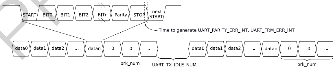
Figure 24-5. Structure of UART Data Frame
