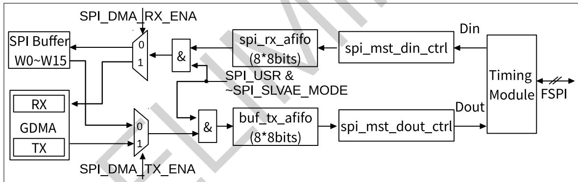
Figure 25-4. Data Flow Control in GP-SPI2 Master Mode
