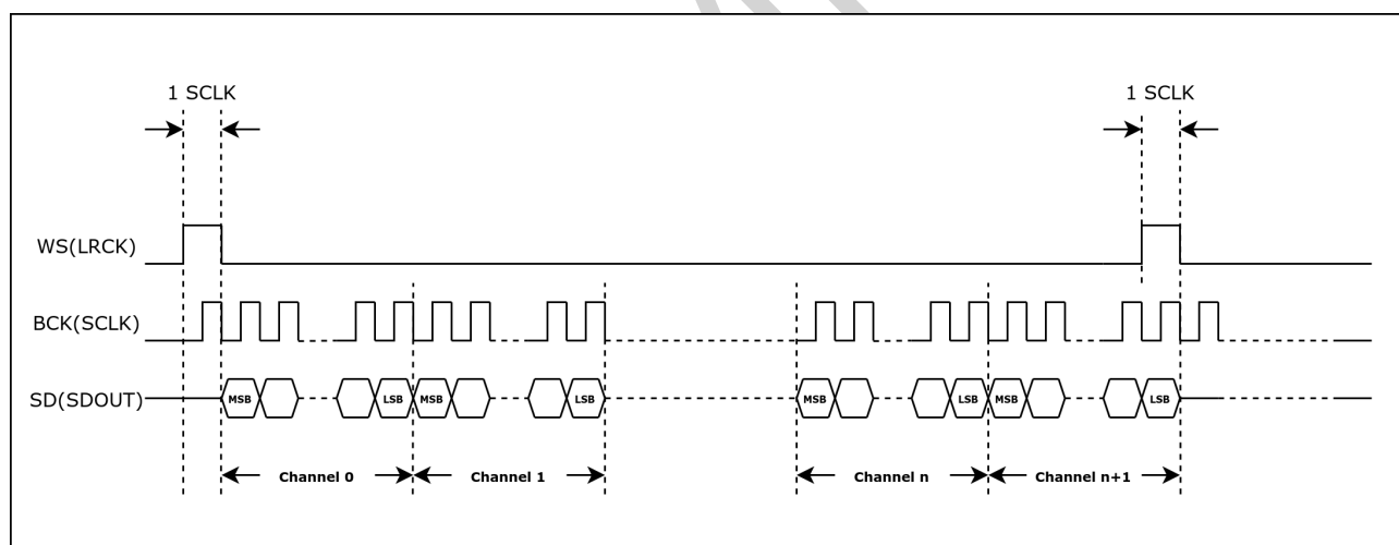
Figure 27-4. TDM PCM Standard Timing Diagram
