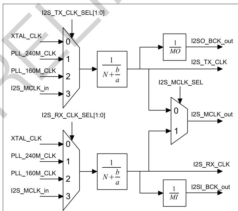
Figure 27-6. I2S Clock
